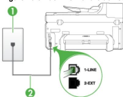
Figure 10-5 Back view of the device
