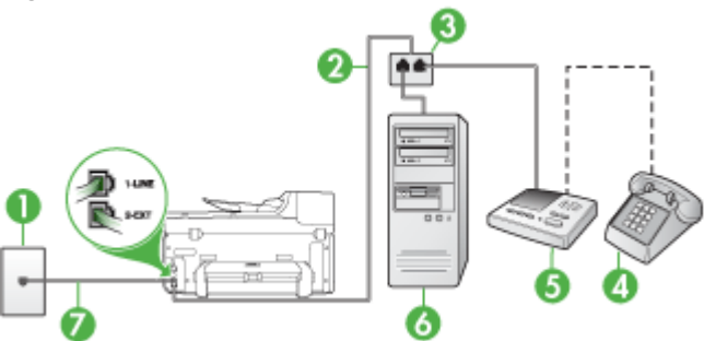
Figure 10-11 Back view of the device
