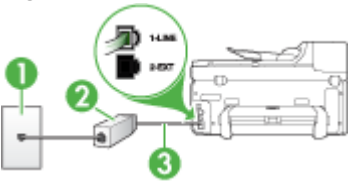
Figure 10-2 Back view of the device
